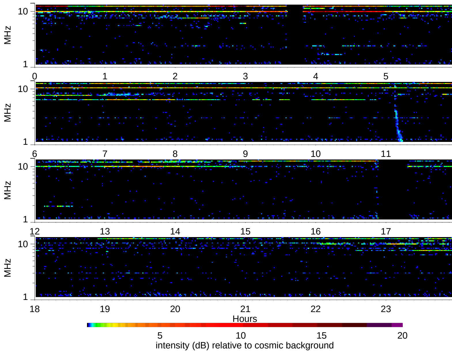
Wind Waves RAD2 receiver: 2005/8/17
