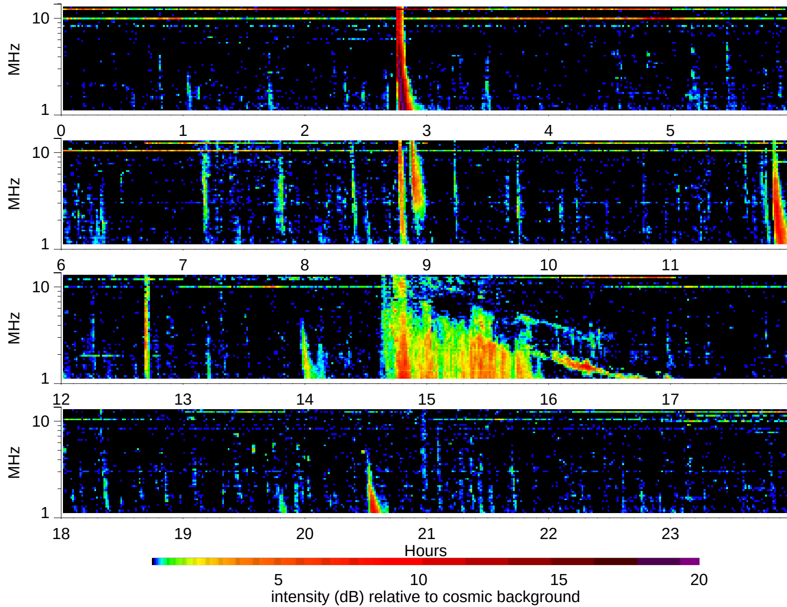
Wind Waves RAD2 receiver: 2005/8/23
