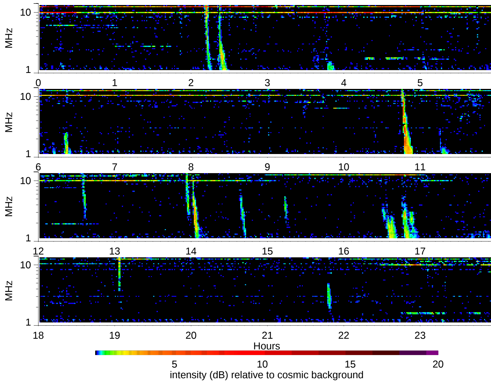
Wind Waves RAD2 receiver: 2005/8/27
