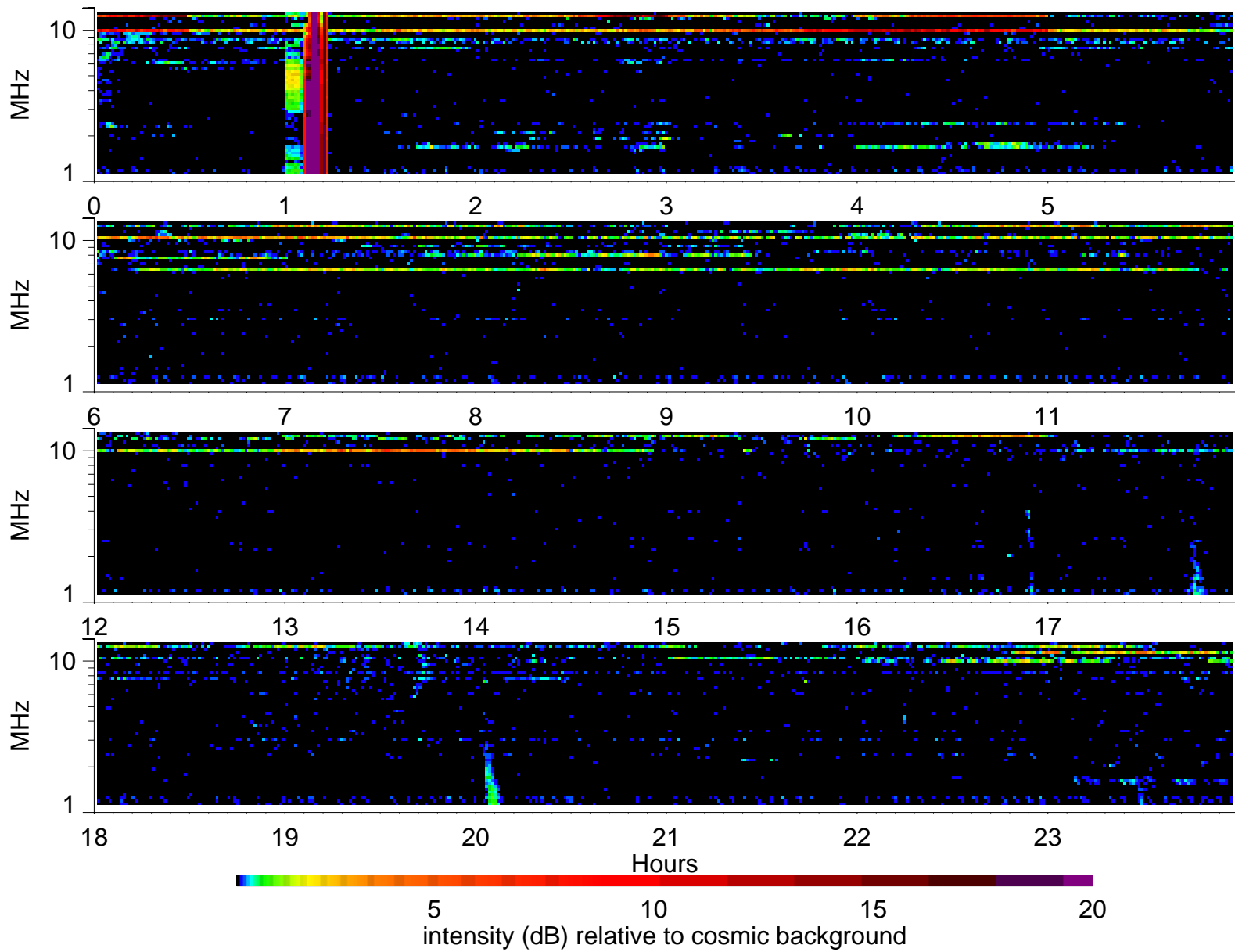
Wind Waves RAD2 receiver: 2005/9/1
