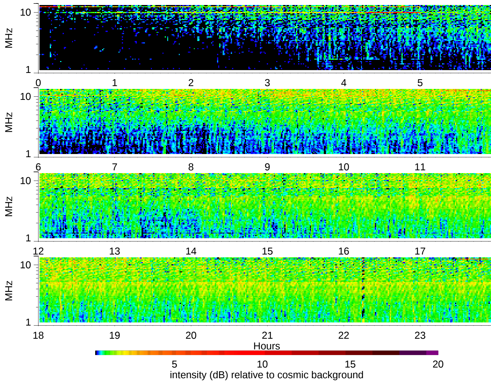
Wind Waves RAD2 receiver: 2005/9/14
