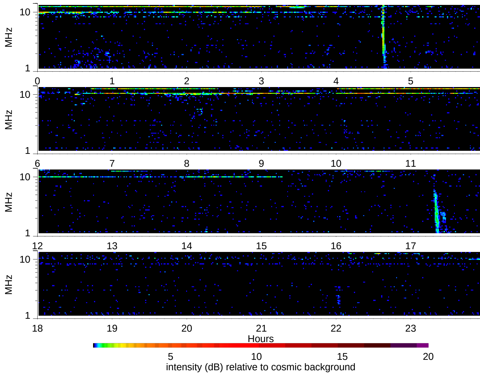
Wind Waves RAD2 receiver: 2005/9/28
