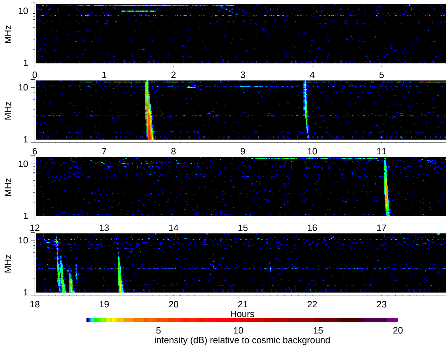
Wind Waves RAD2 receiver: 2005/10/10
