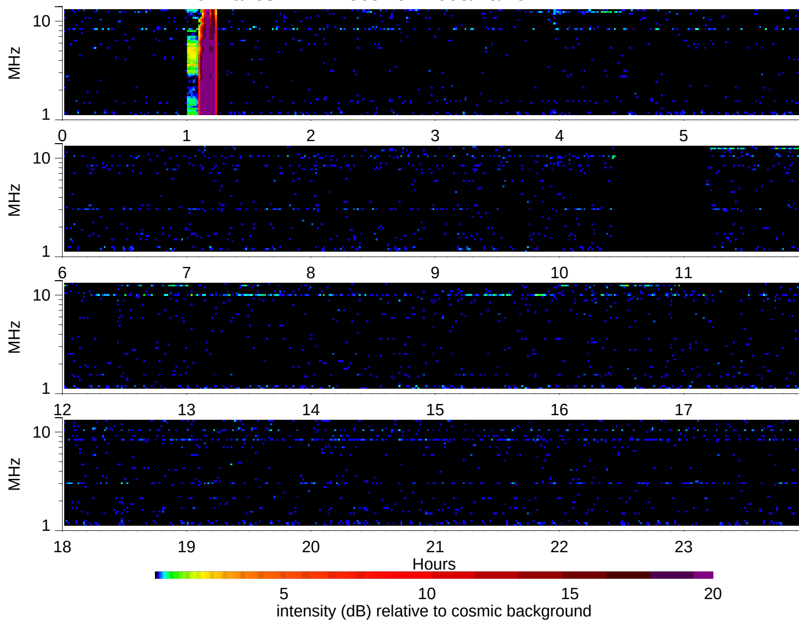
Wind Waves RAD2 receiver: 2005/10/29
