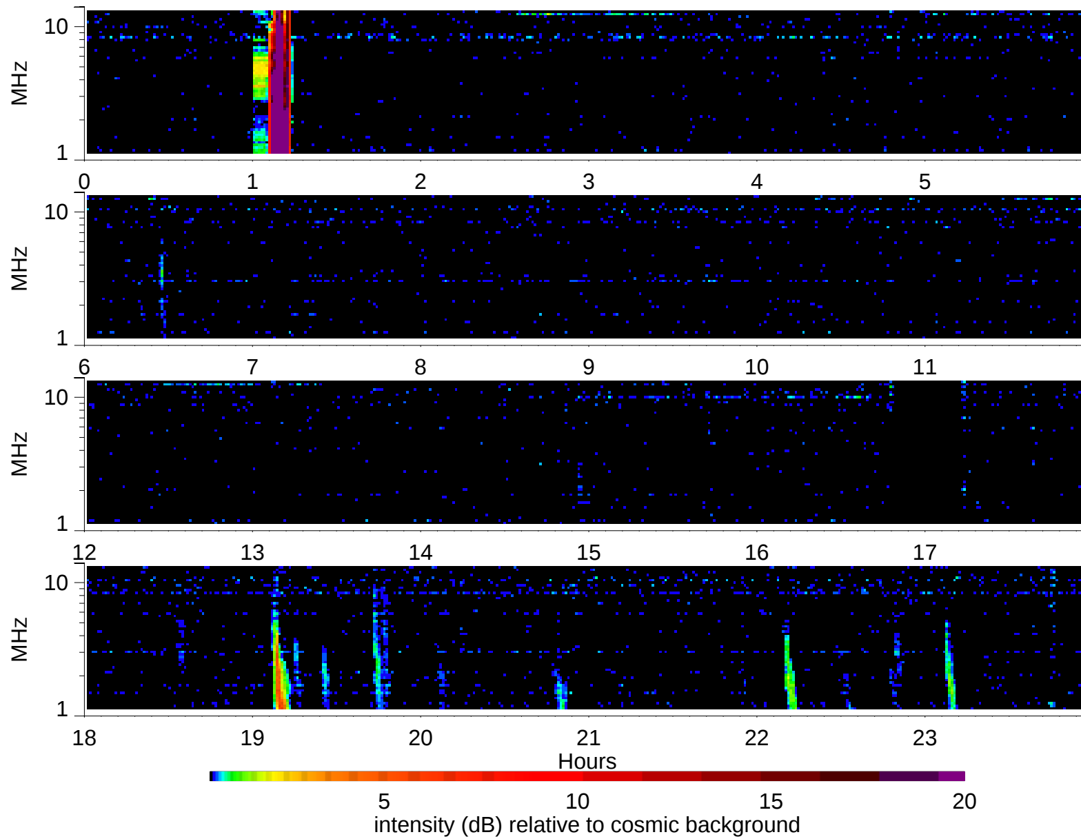
Wind Waves RAD2 receiver: 2005/10/31
