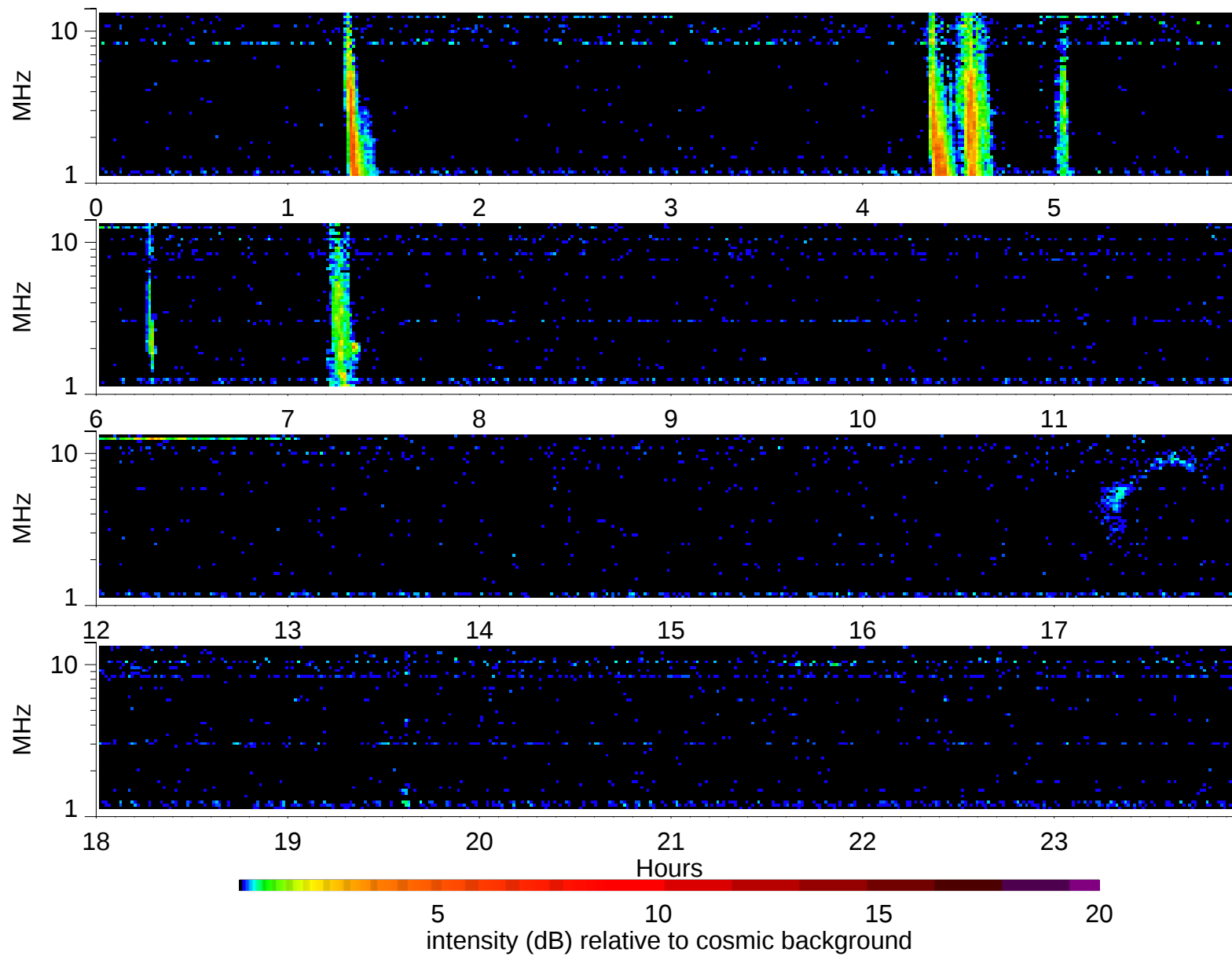
Wind Waves RAD2 receiver: 2005/11/3
