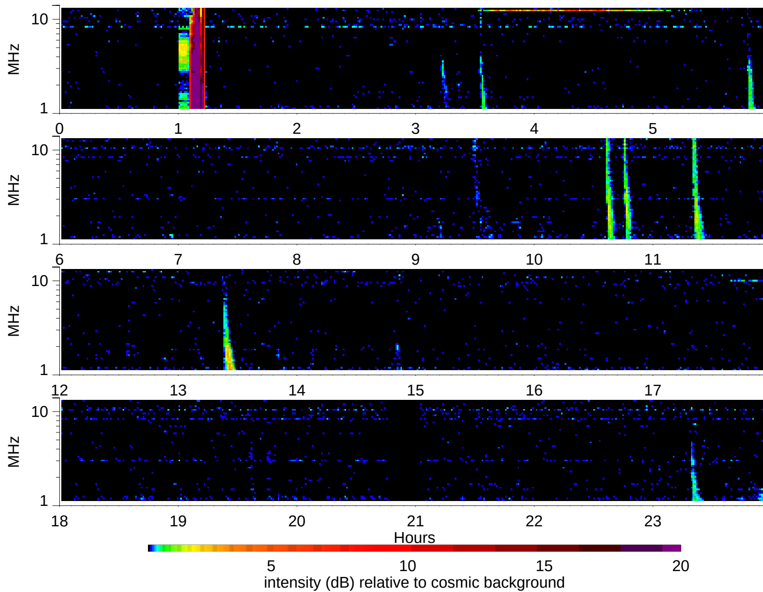
Wind Waves RAD2 receiver: 2005/11/8
