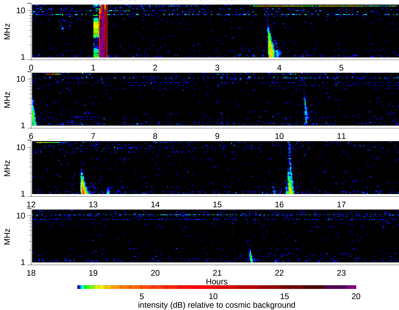
Wind Waves RAD2 receiver: 2005/11/24
