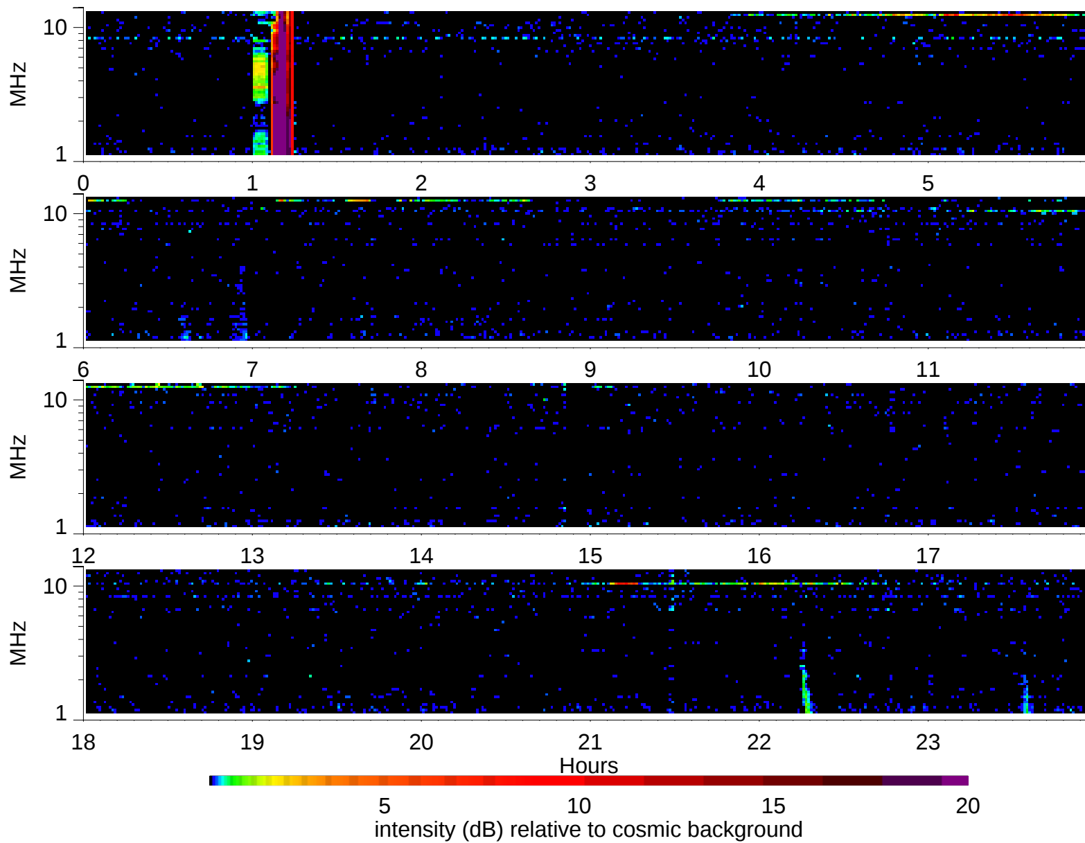
Wind Waves RAD2 receiver: 2005/11/26
