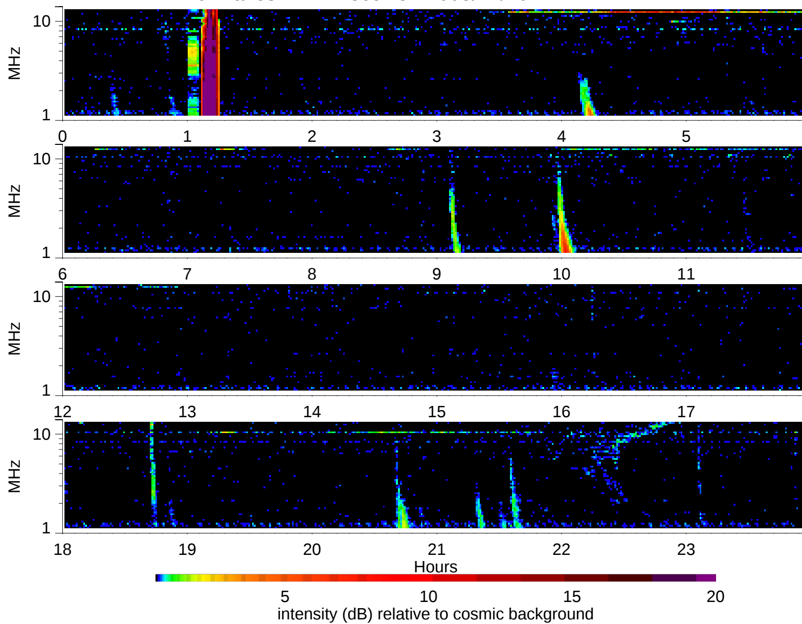
Wind Waves RAD2 receiver: 2005/12/10
