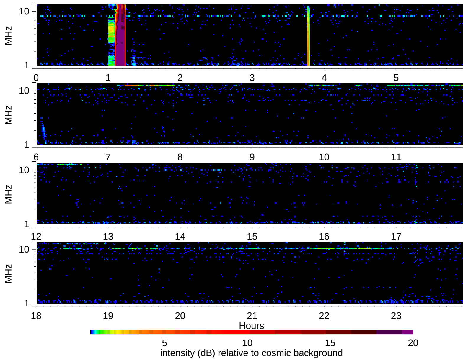
Wind Waves RAD2 receiver: 2005/12/14
