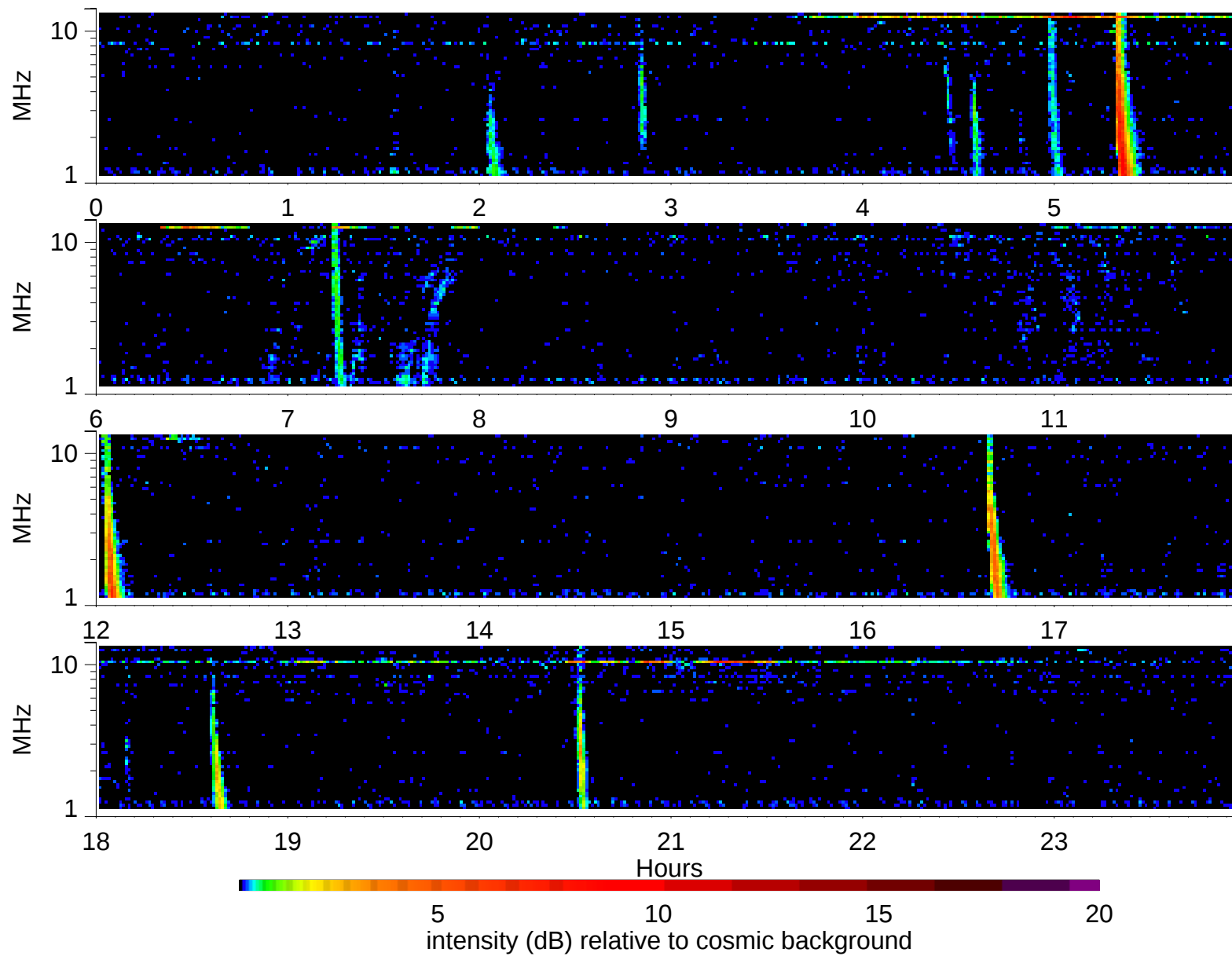
Wind Waves RAD2 receiver: 2005/12/15
