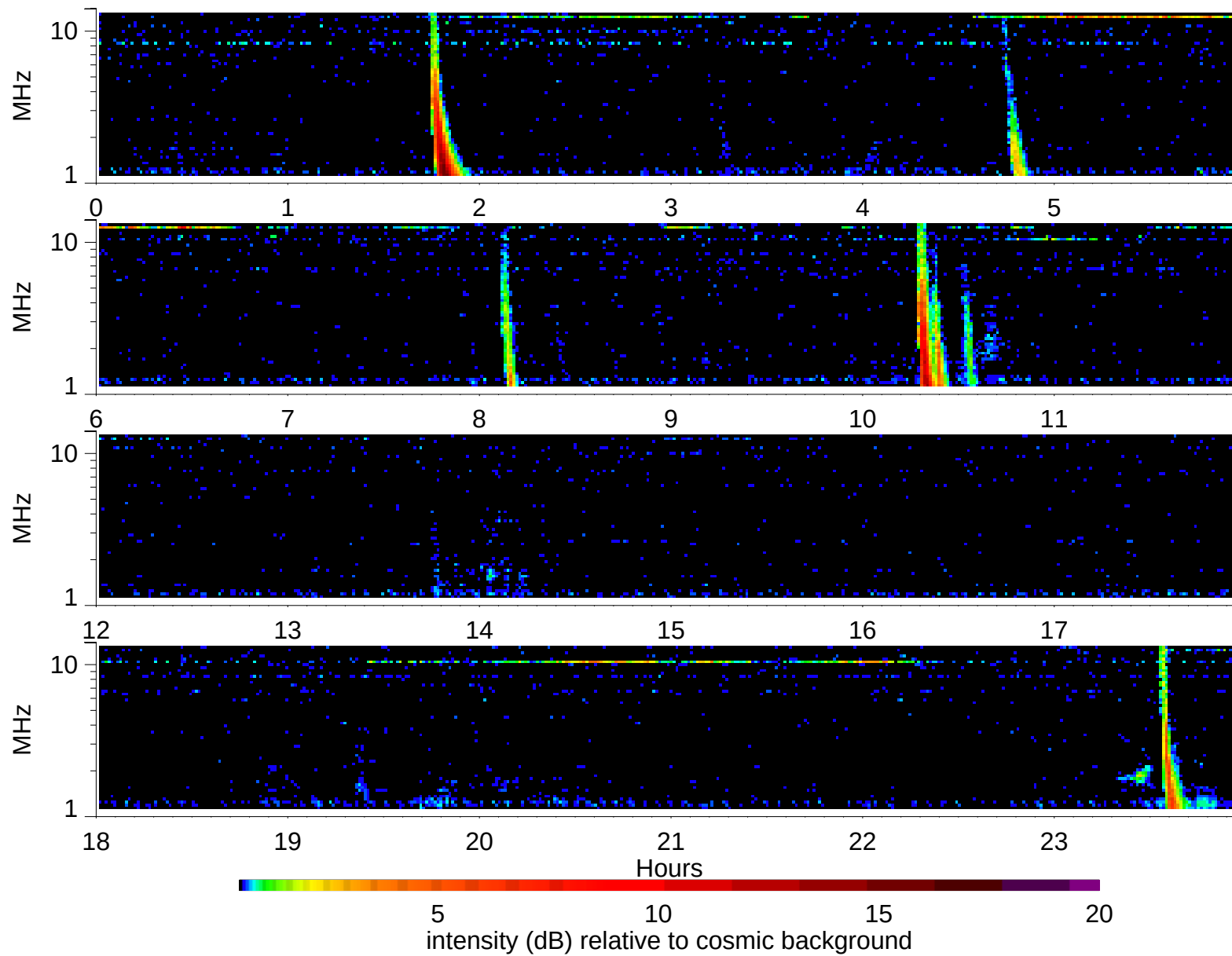
Wind Waves RAD2 receiver: 2005/12/21
