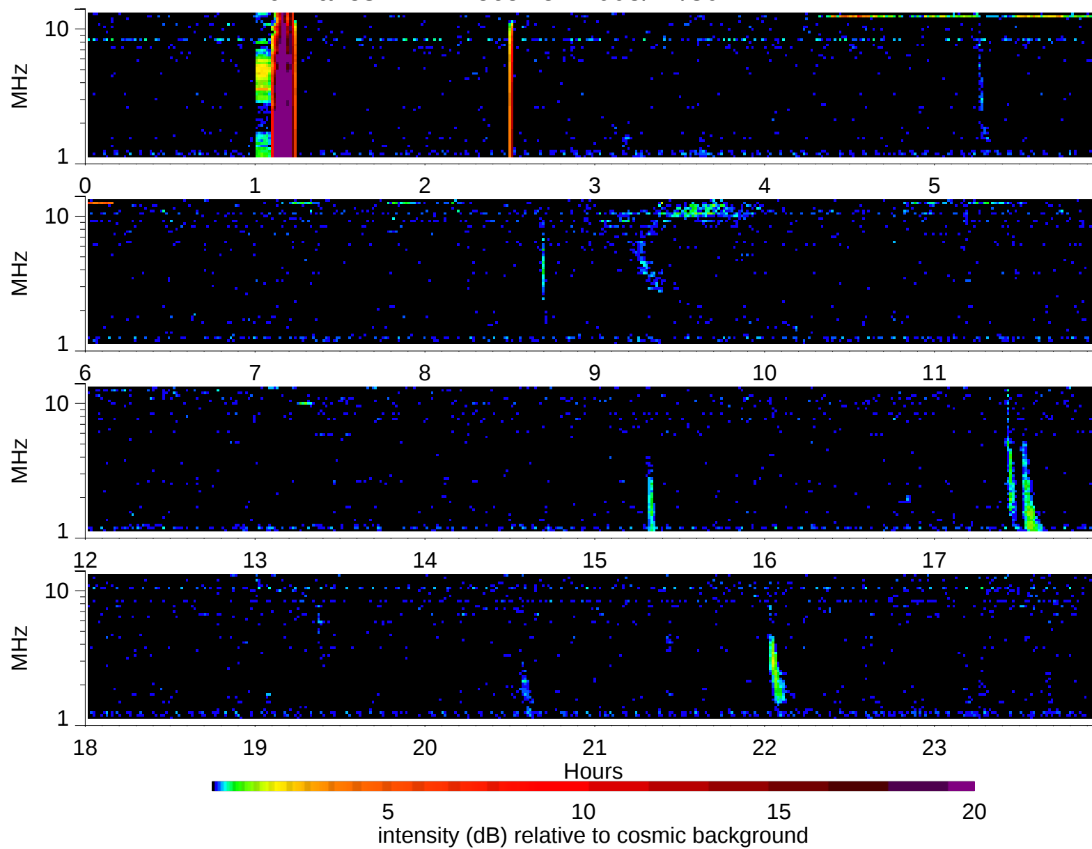
Wind Waves RAD2 receiver: 2005/12/30
