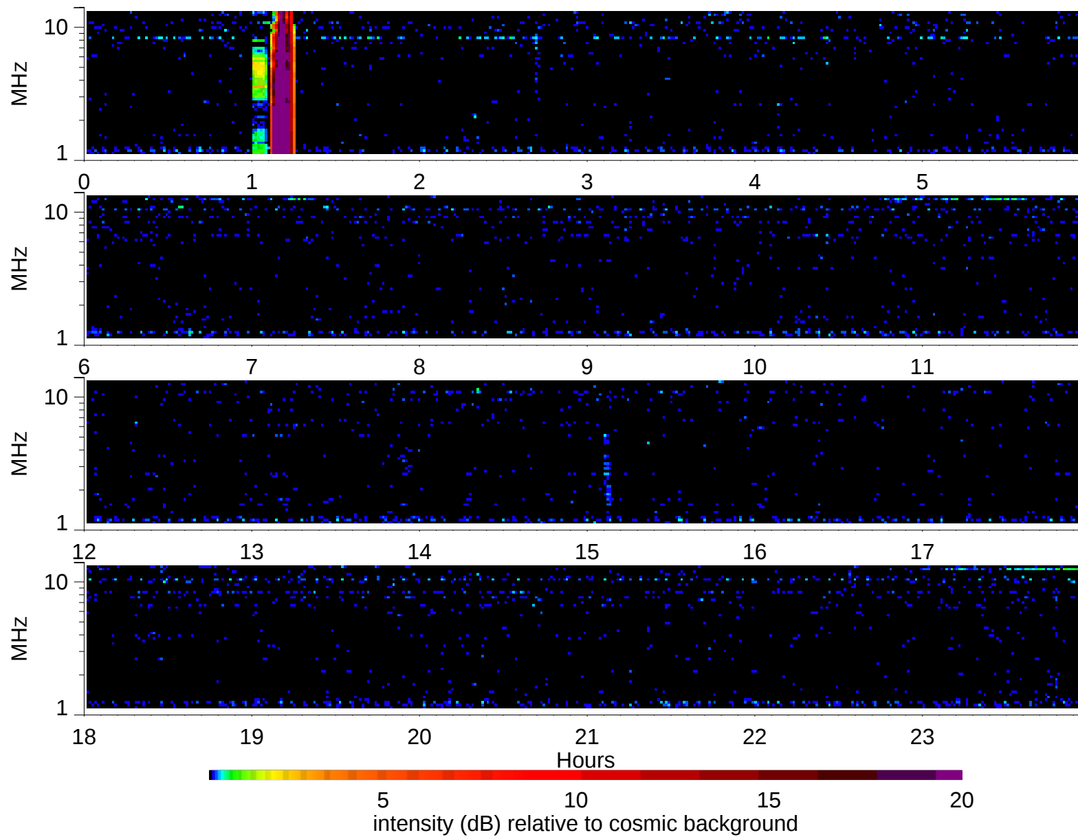
Wind Waves RAD2 receiver: 2006/1/2
