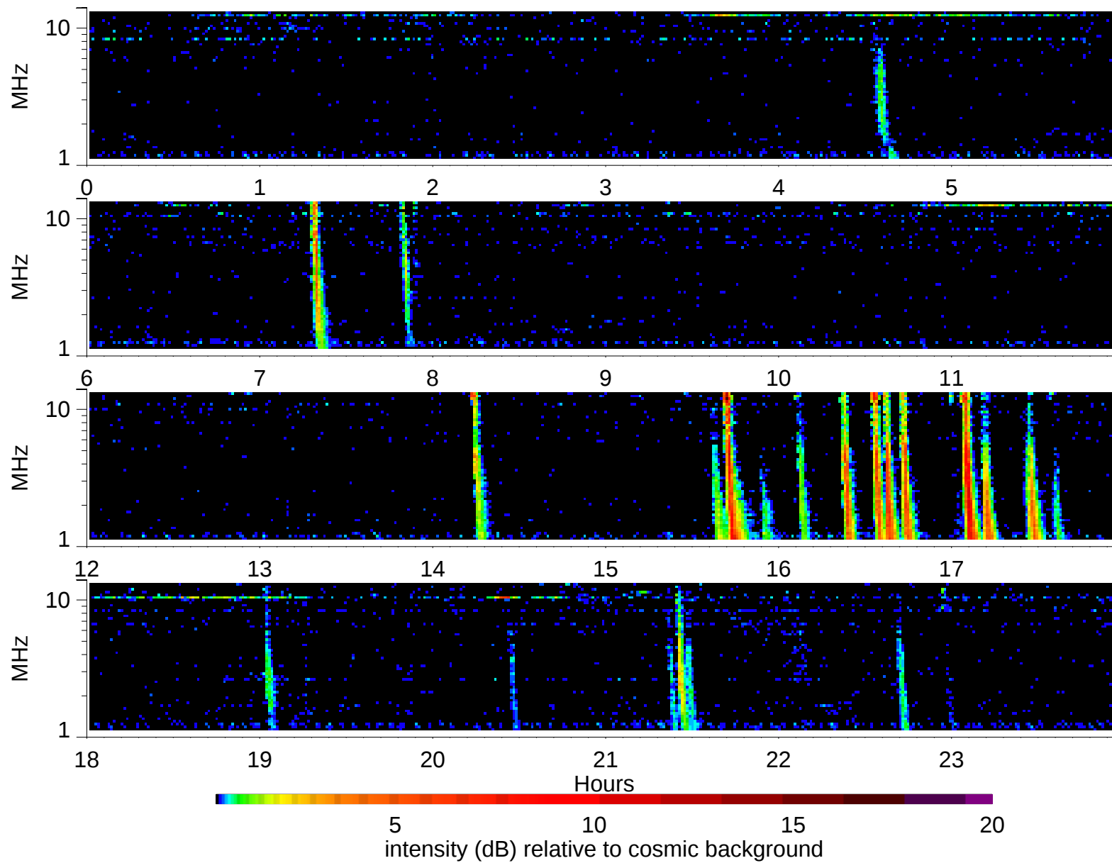
Wind Waves RAD2 receiver: 2006/1/3
