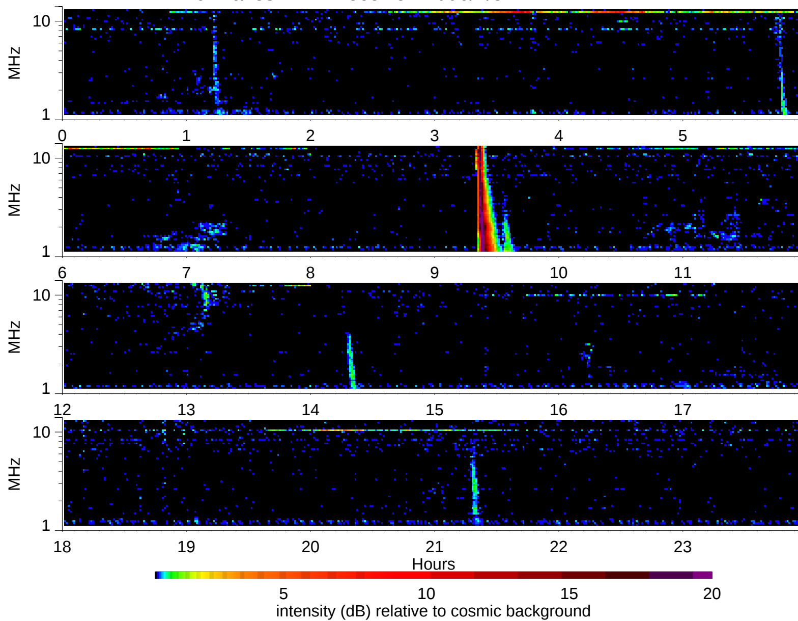
Wind Waves RAD2 receiver: 2006/1/5
