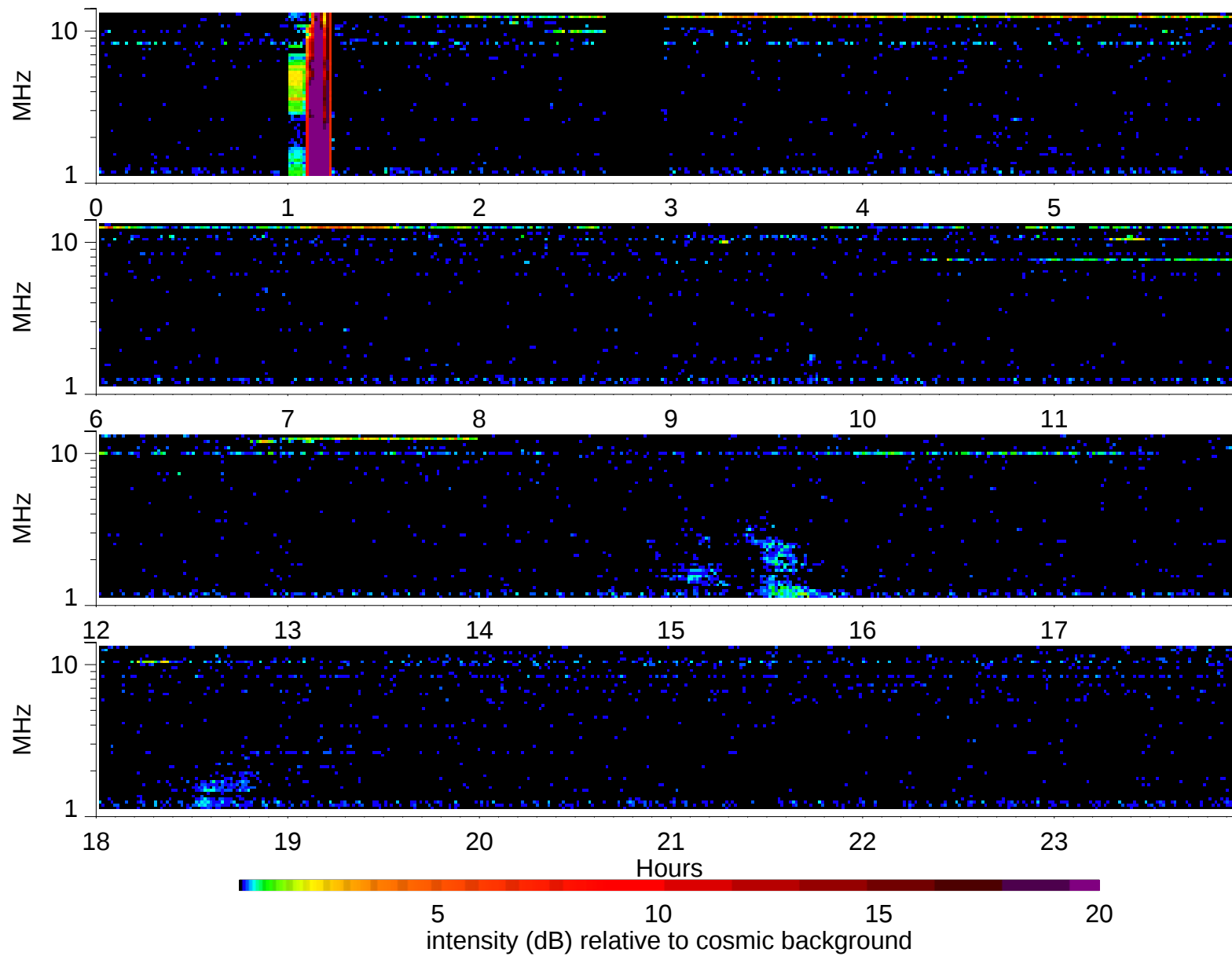
Wind Waves RAD2 receiver: 2006/1/8
