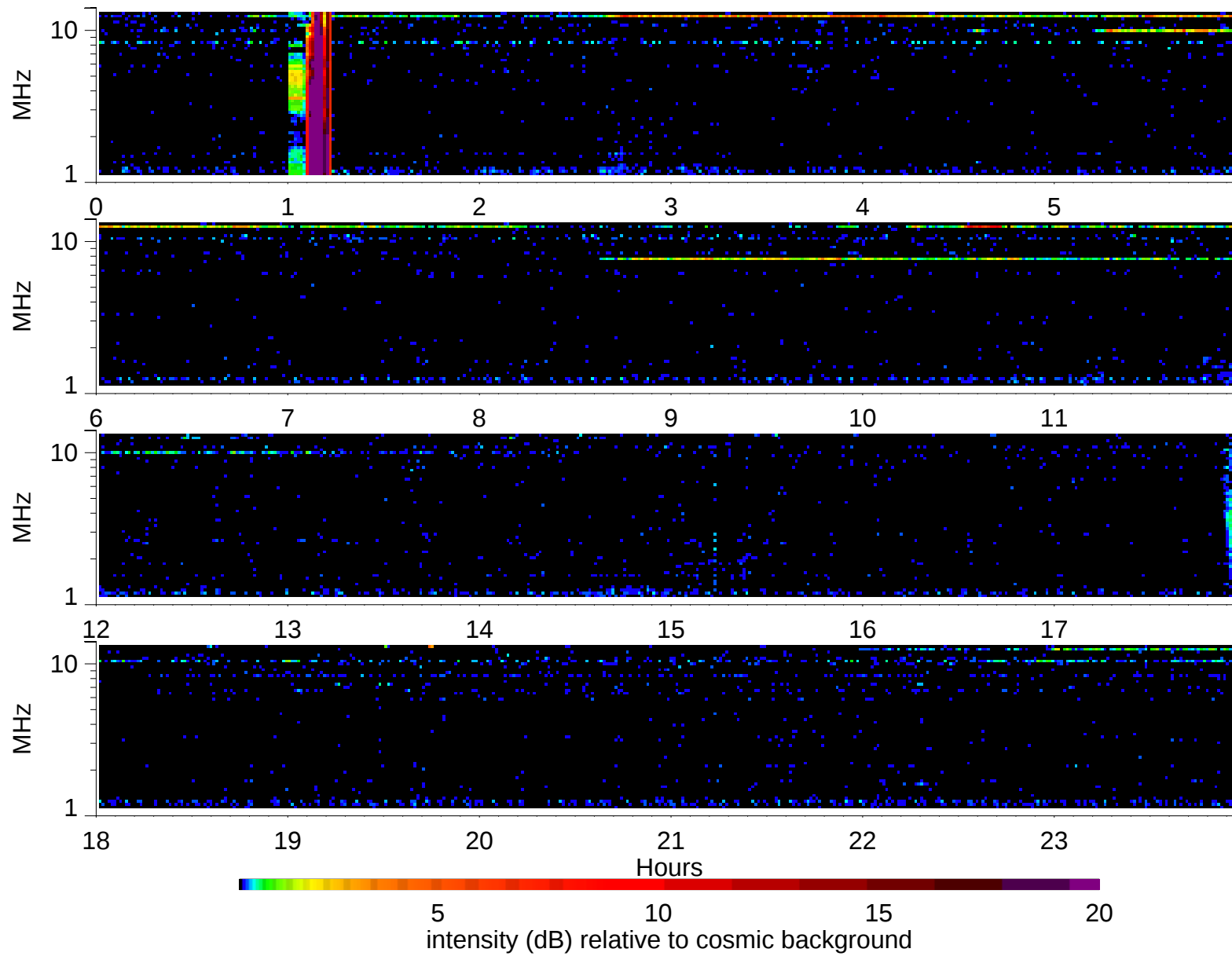
Wind Waves RAD2 receiver: 2006/1/16
