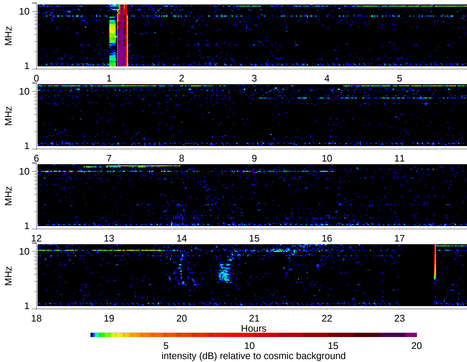
Wind Waves RAD2 receiver: 2006/1/18
