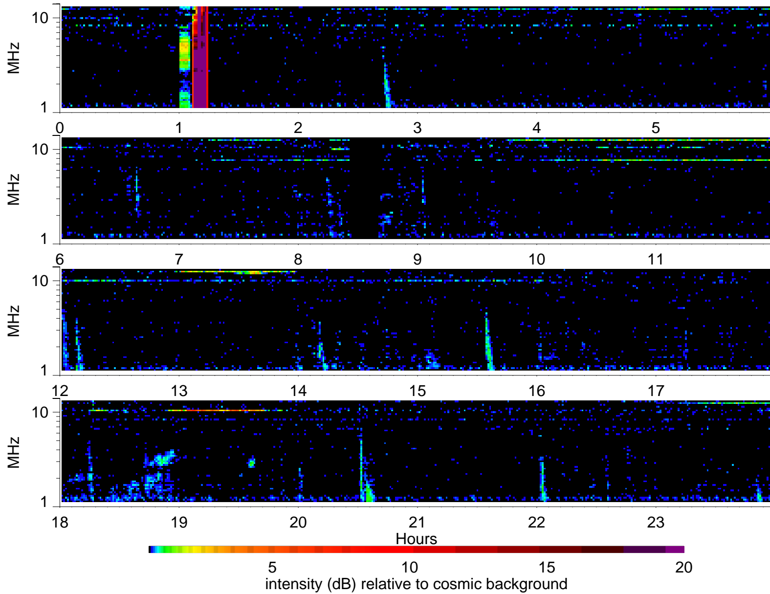
Wind Waves RAD2 receiver: 2006/1/20
