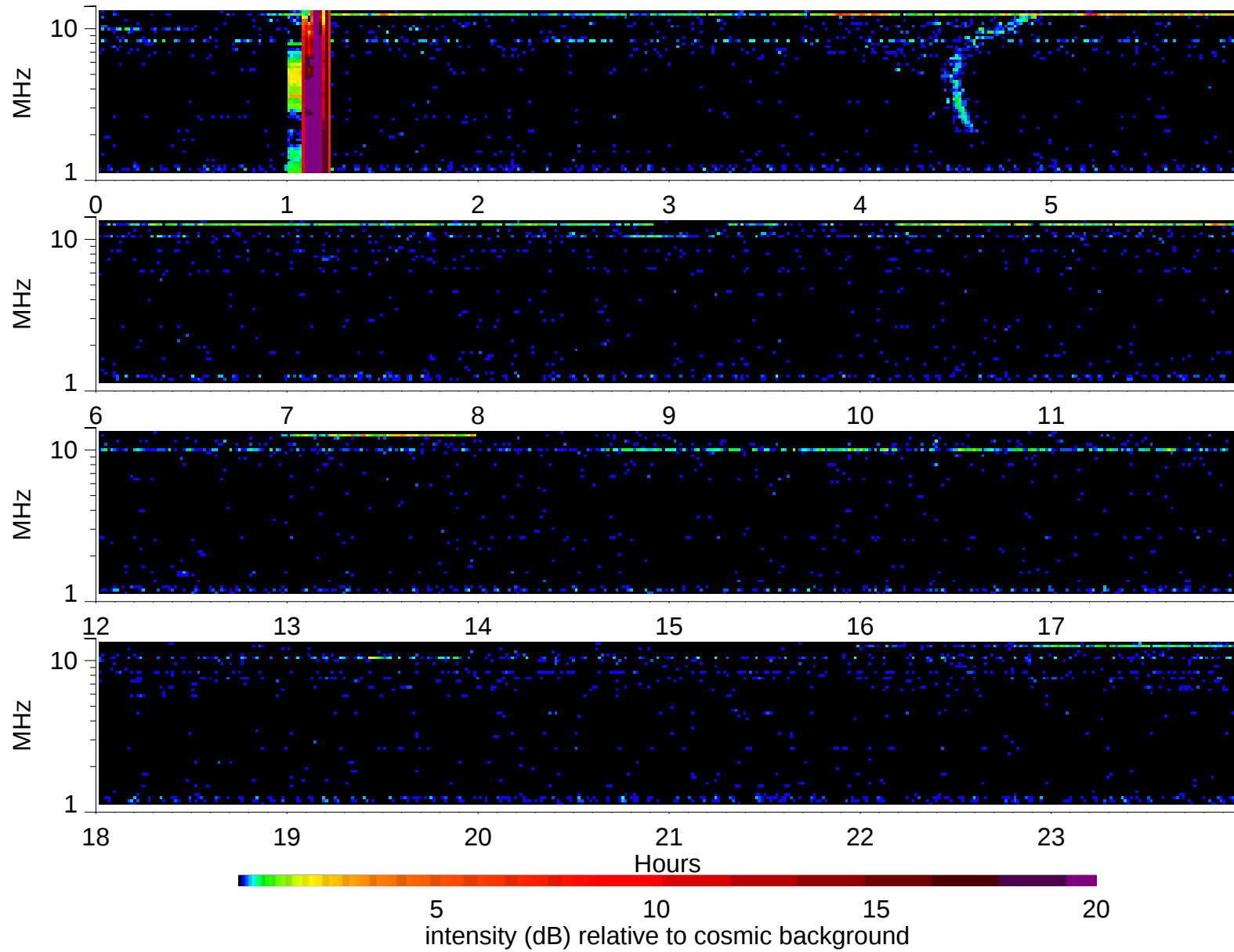
Wind Waves RAD2 receiver: 2006/1/24
