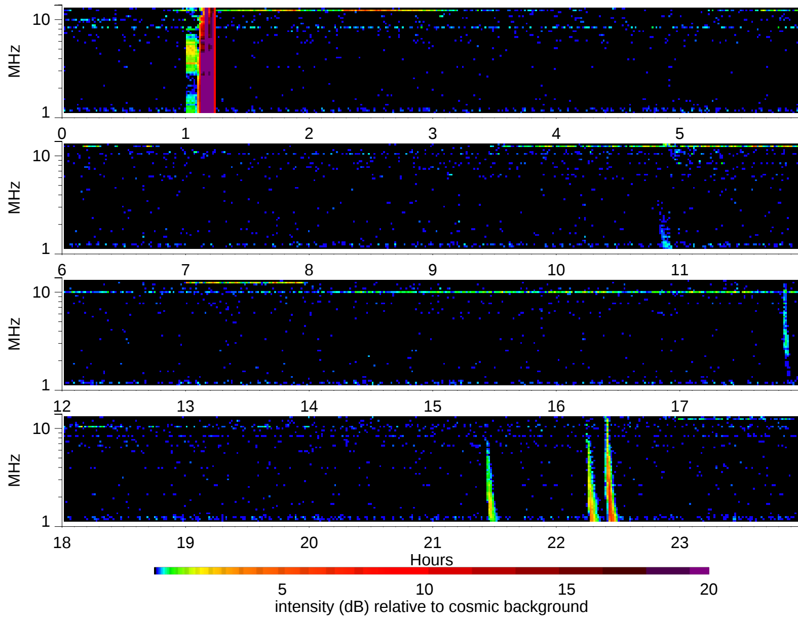
Wind Waves RAD2 receiver: 2006/1/28
