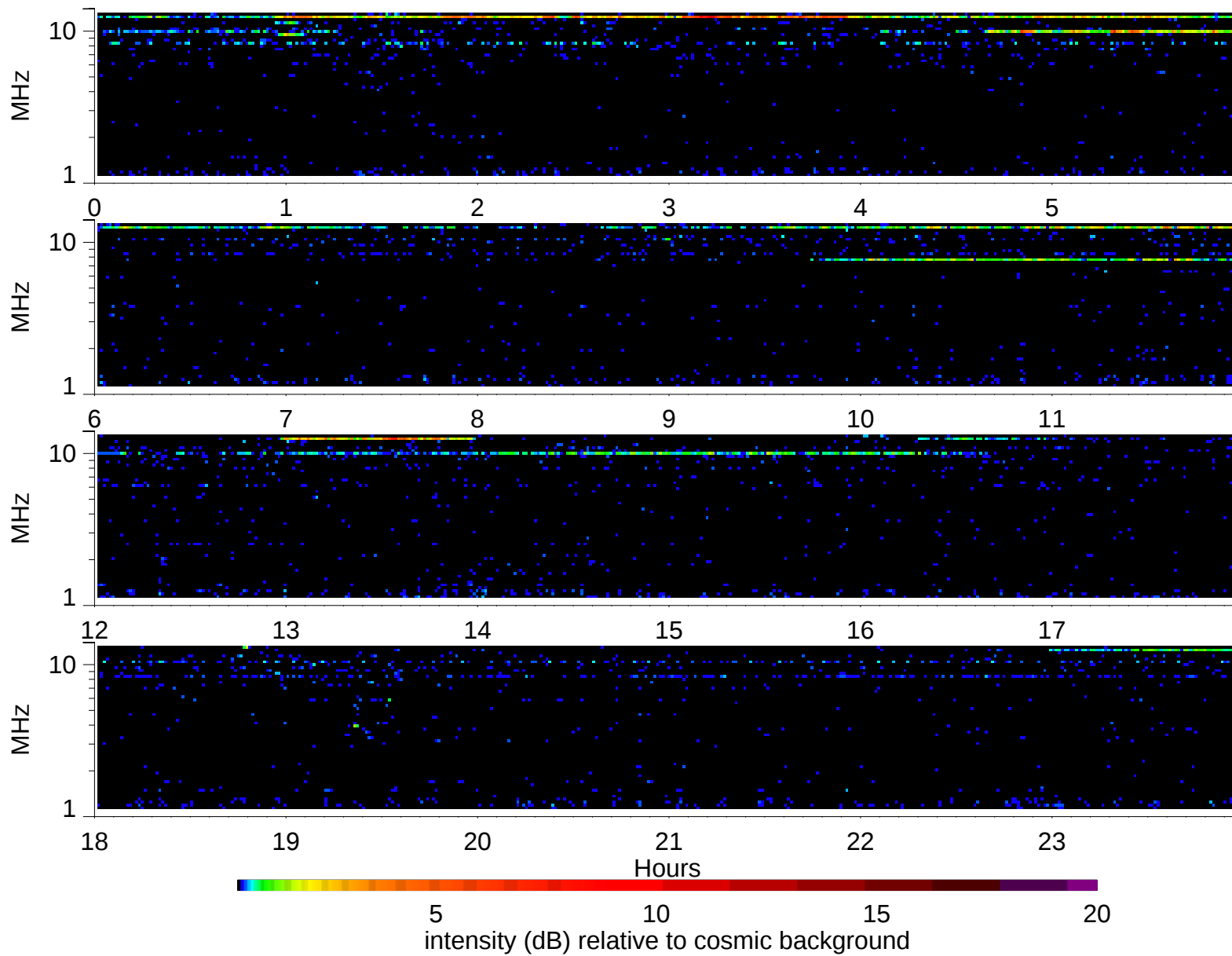
Wind Waves RAD2 receiver: 2006/2/2
