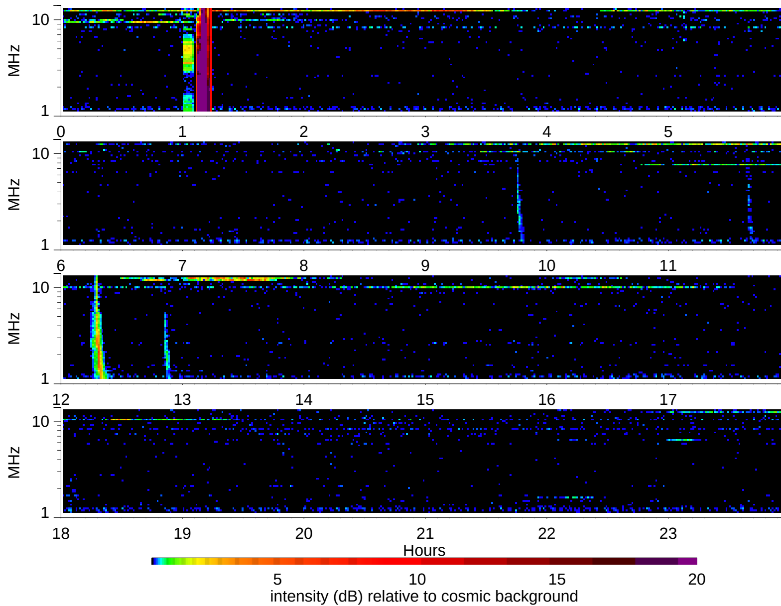
Wind Waves RAD2 receiver: 2006/2/3
