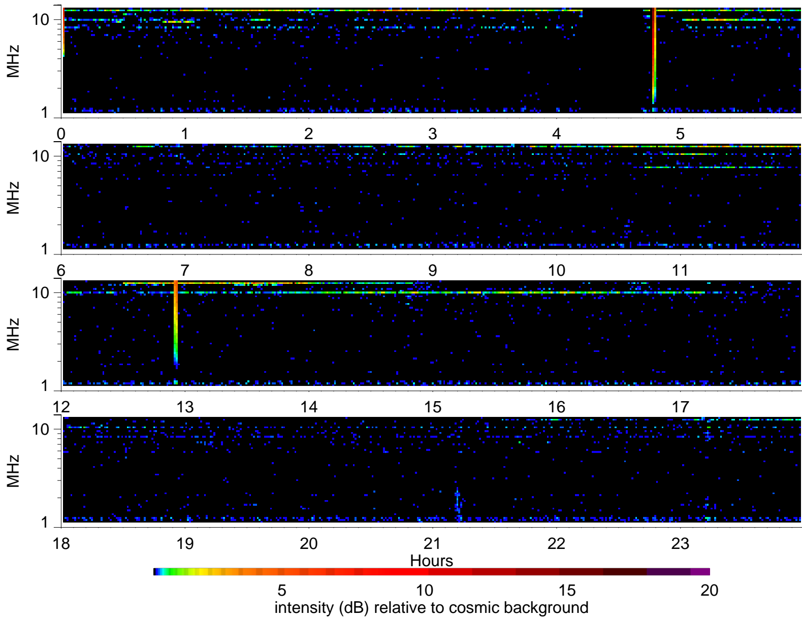
Wind Waves RAD2 receiver: 2006/2/4
