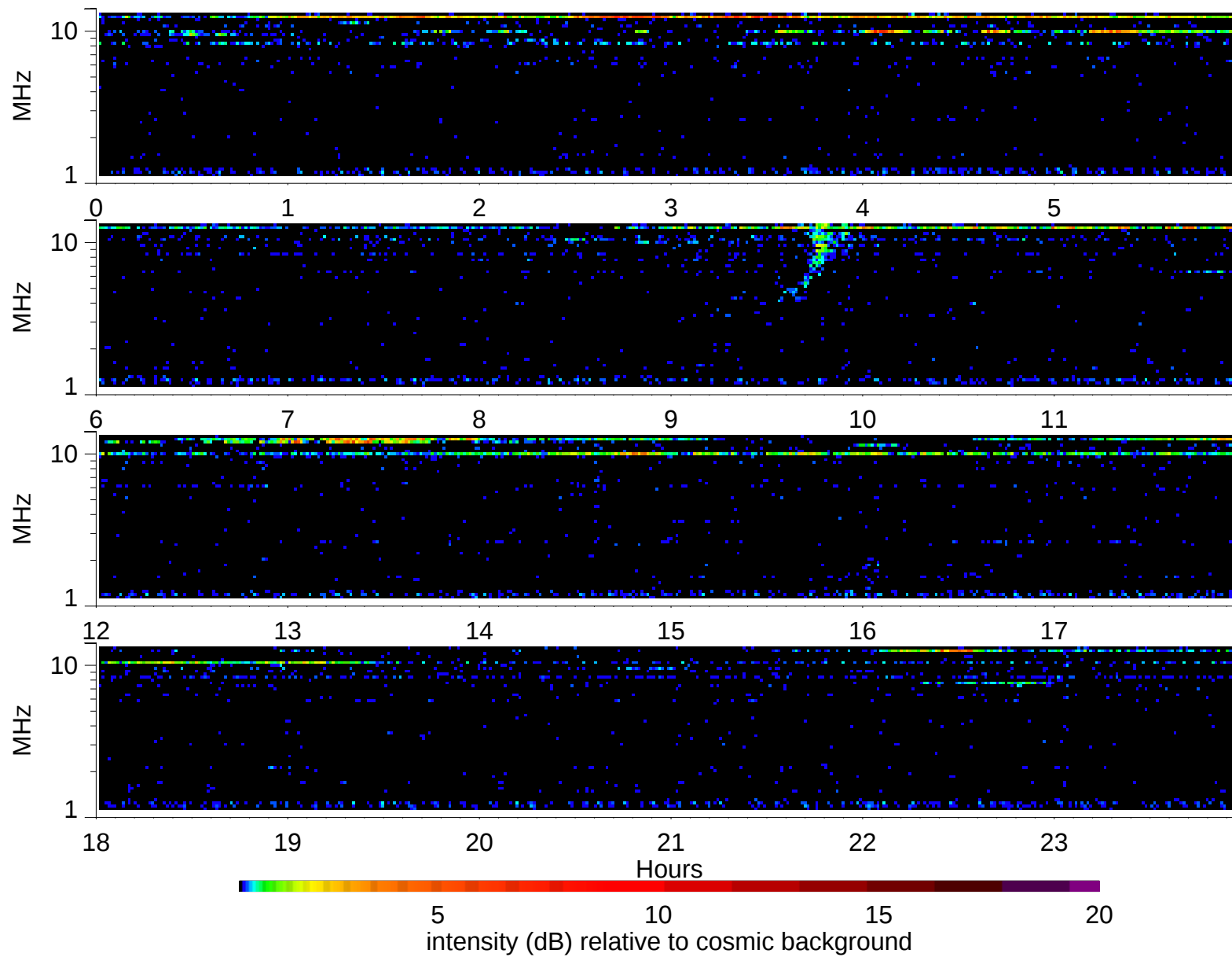
Wind Waves RAD2 receiver: 2006/2/6
