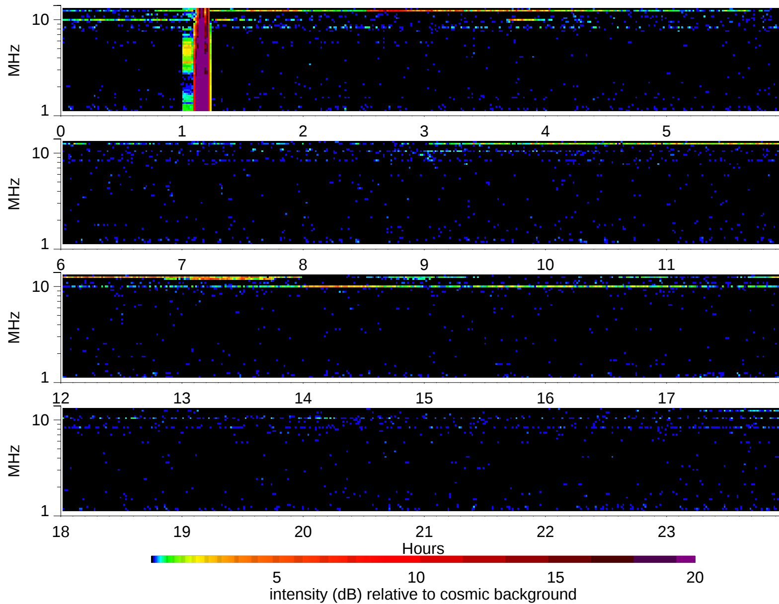
Wind Waves RAD2 receiver: 2006/2/7
