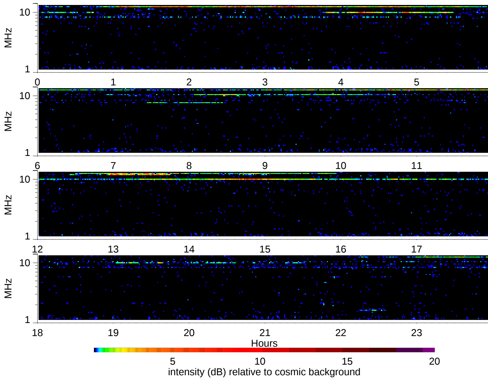
Wind Waves RAD2 receiver: 2006/2/10
