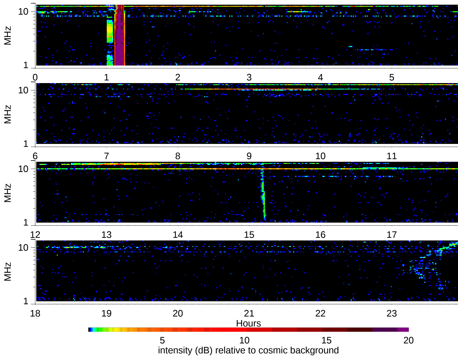
Wind Waves RAD2 receiver: 2006/2/17
