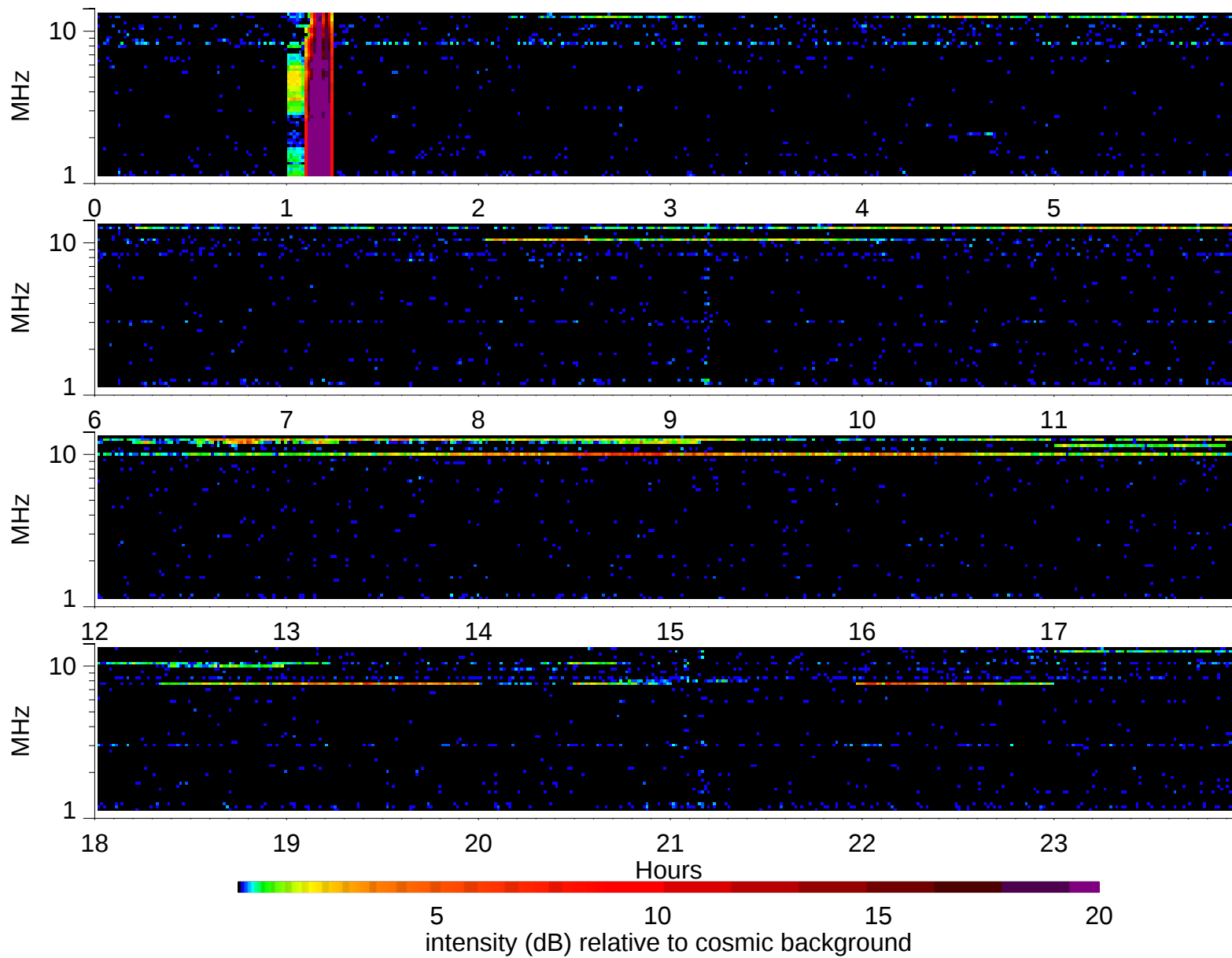
Wind Waves RAD2 receiver: 2006/2/21
