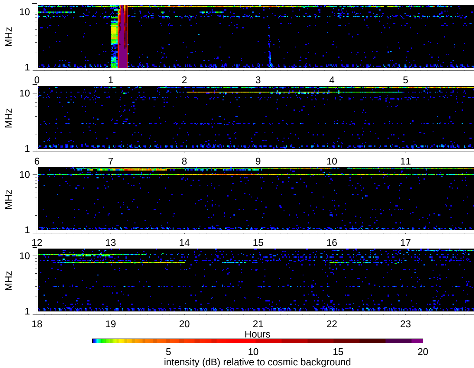
Wind Waves RAD2 receiver: 2006/2/23
