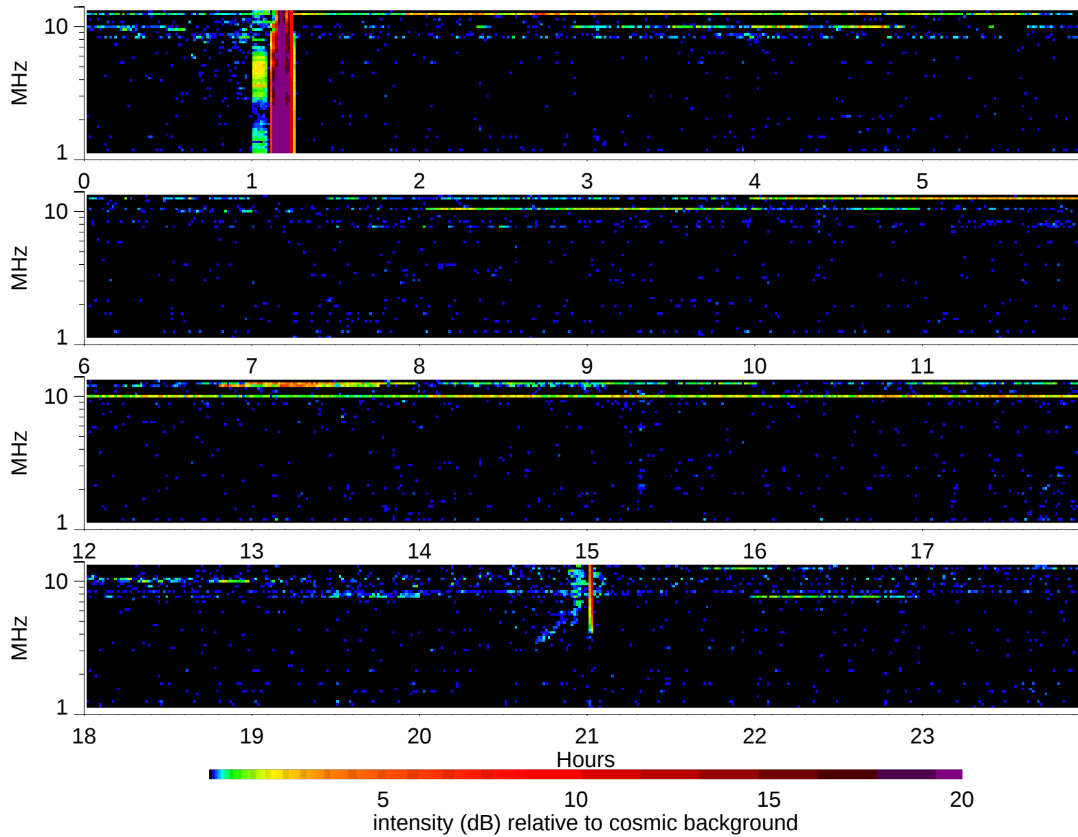
Wind Waves RAD2 receiver: 2006/2/25
