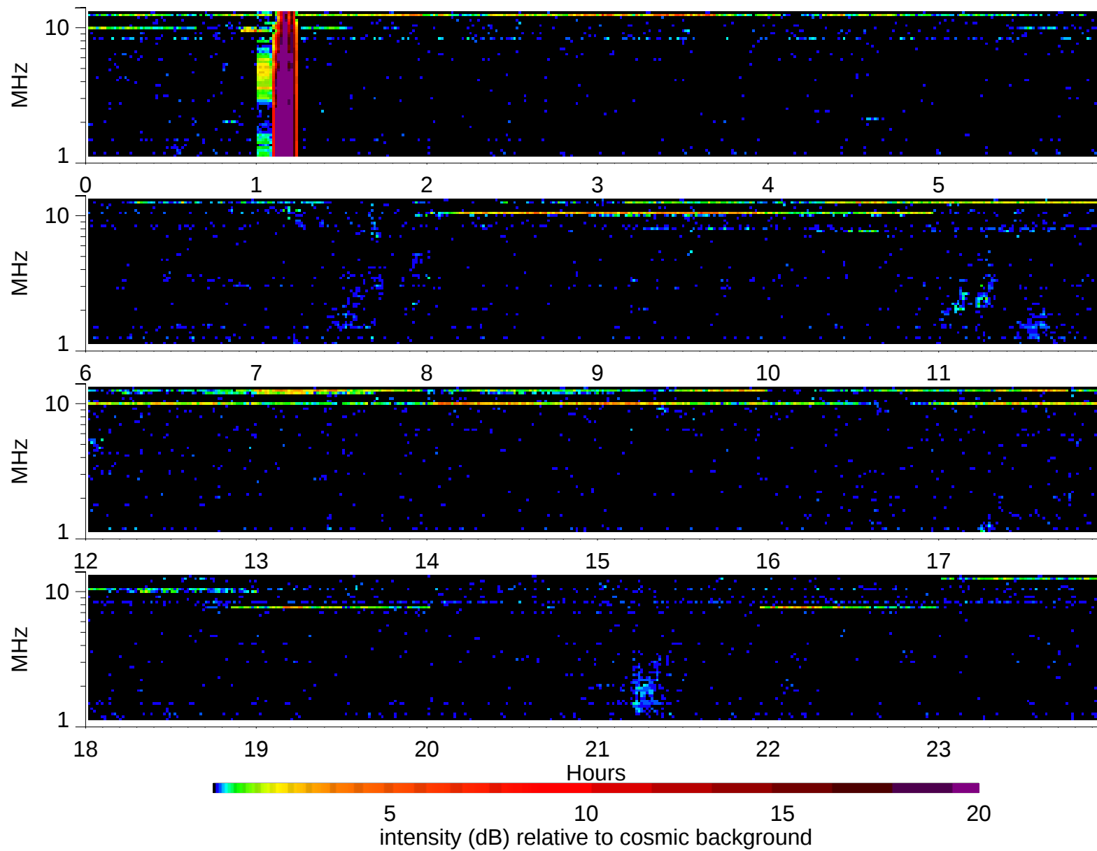
Wind Waves RAD2 receiver: 2006/3/1
