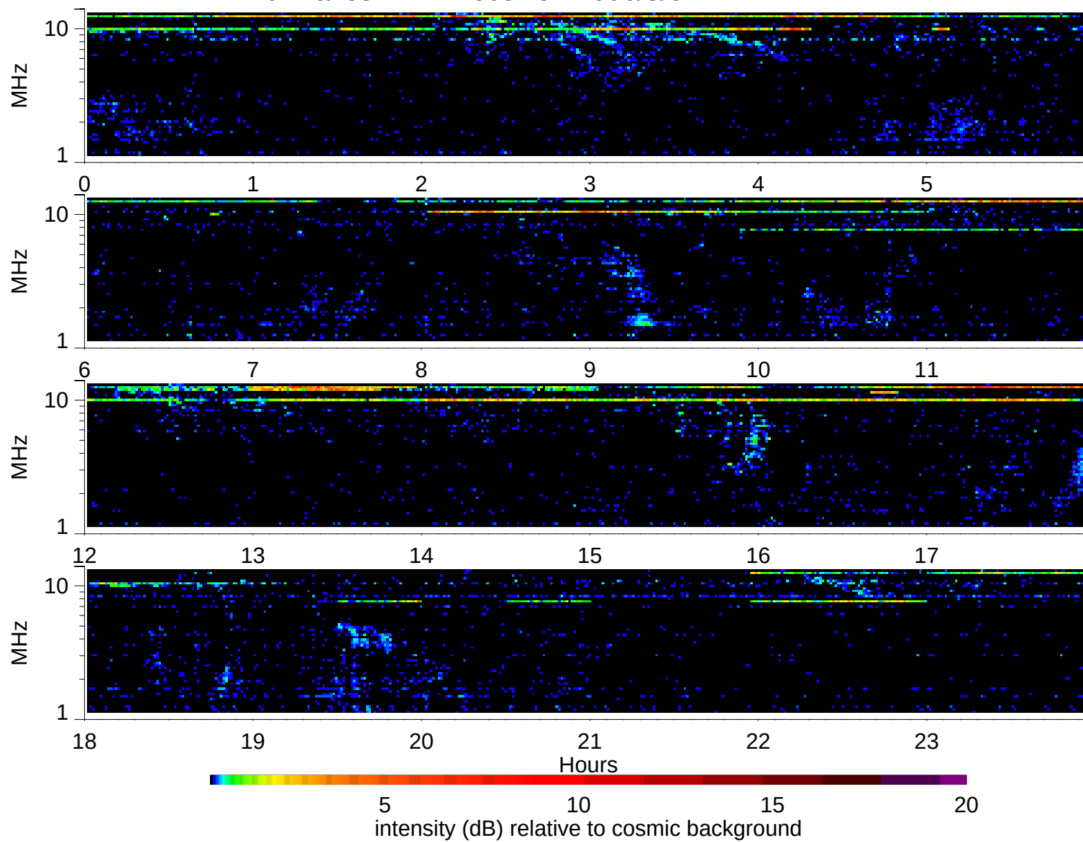
Wind Waves RAD2 receiver: 2006/3/6
