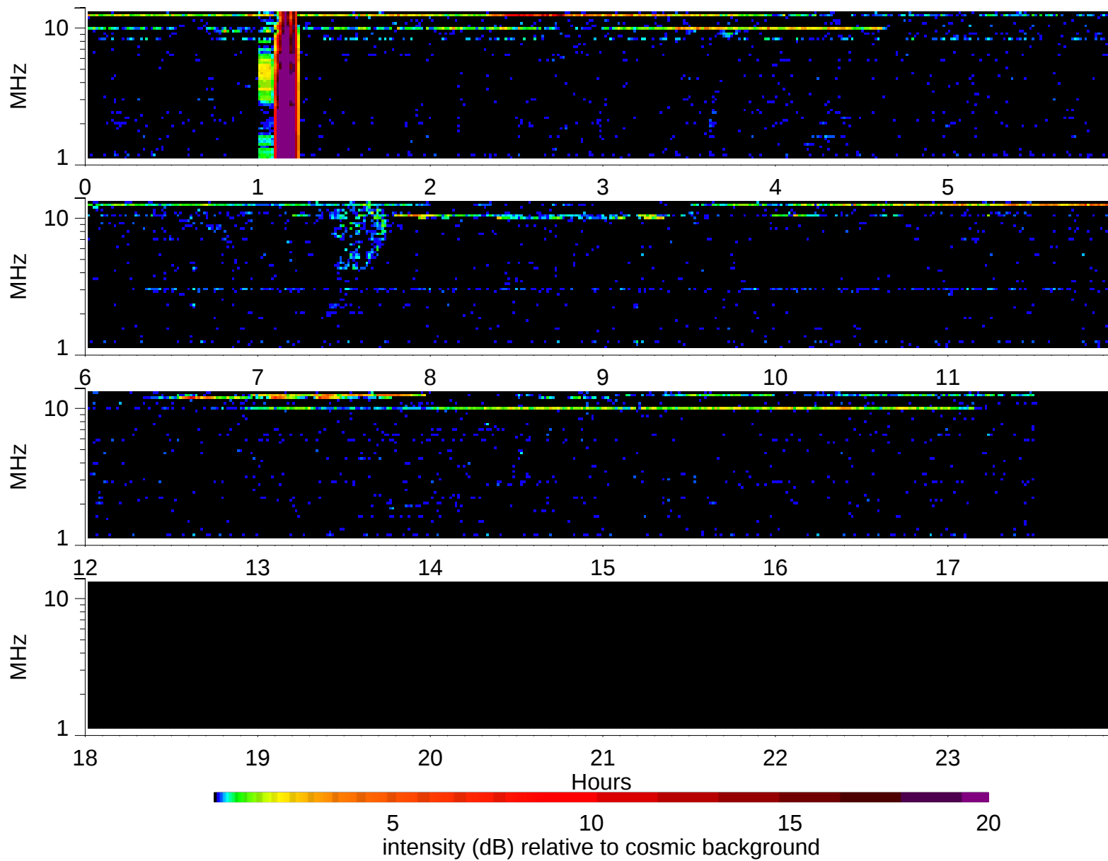
Wind Waves RAD2 receiver: 2006/3/17
