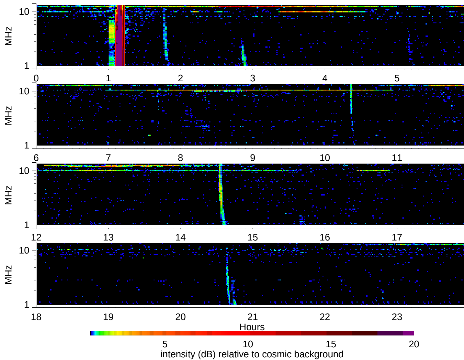
Wind Waves RAD2 receiver: 2006/3/19
