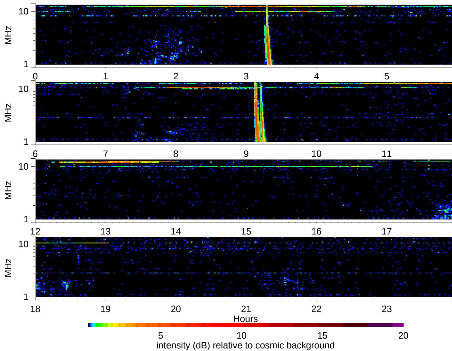
Wind Waves RAD2 receiver: 2006/3/20
