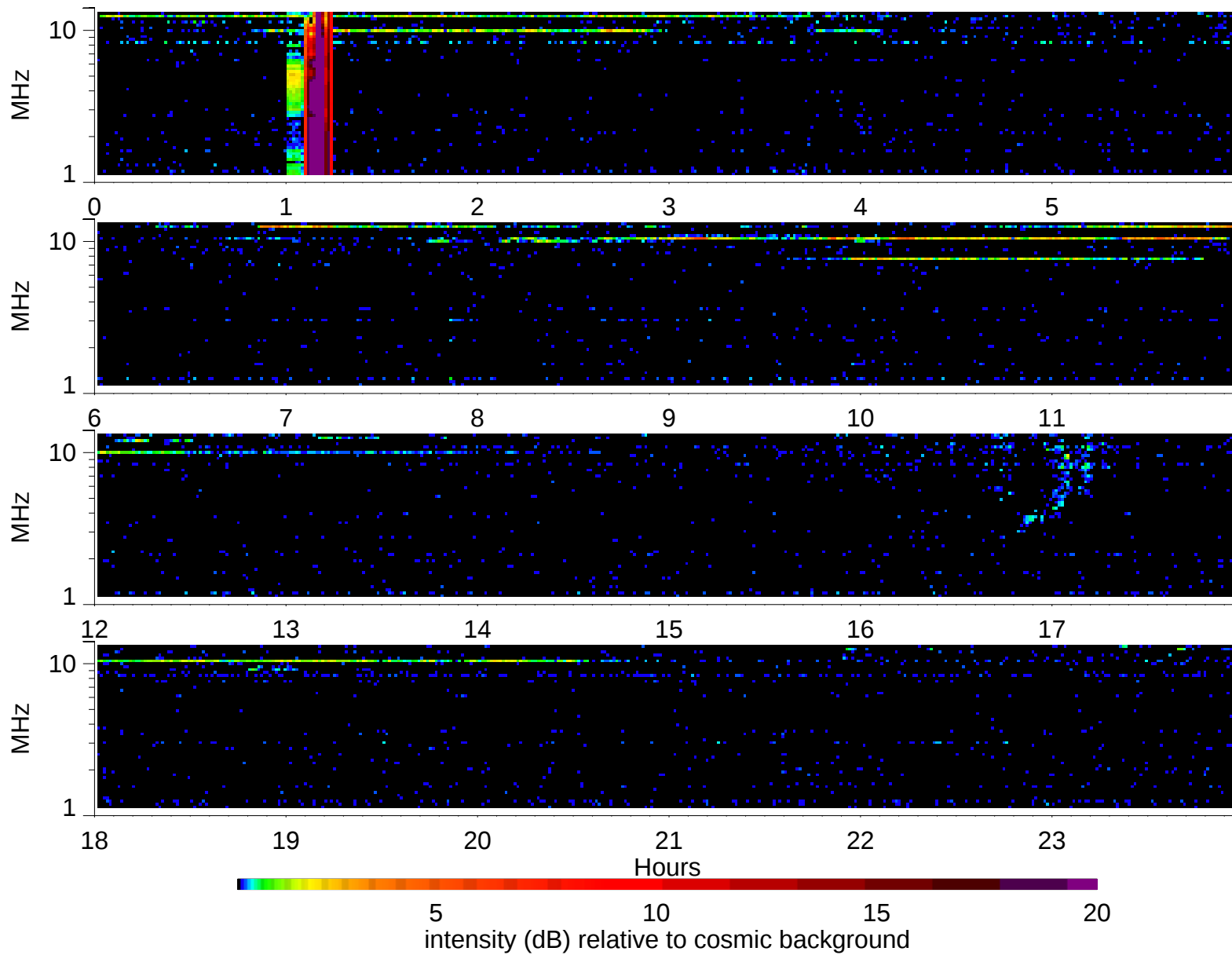
Wind Waves RAD2 receiver: 2006/3/29
