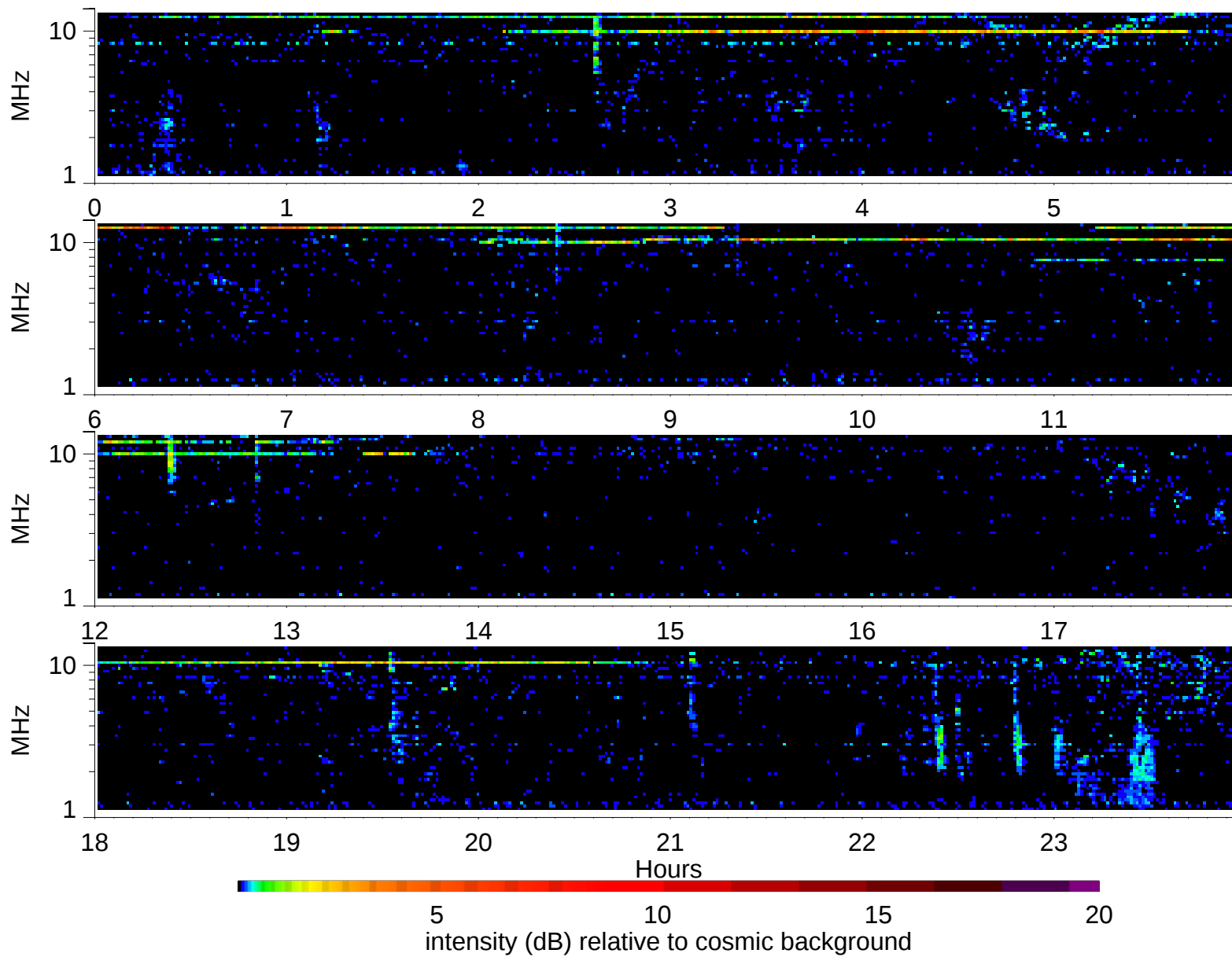
Wind Waves RAD2 receiver: 2006/4/3
