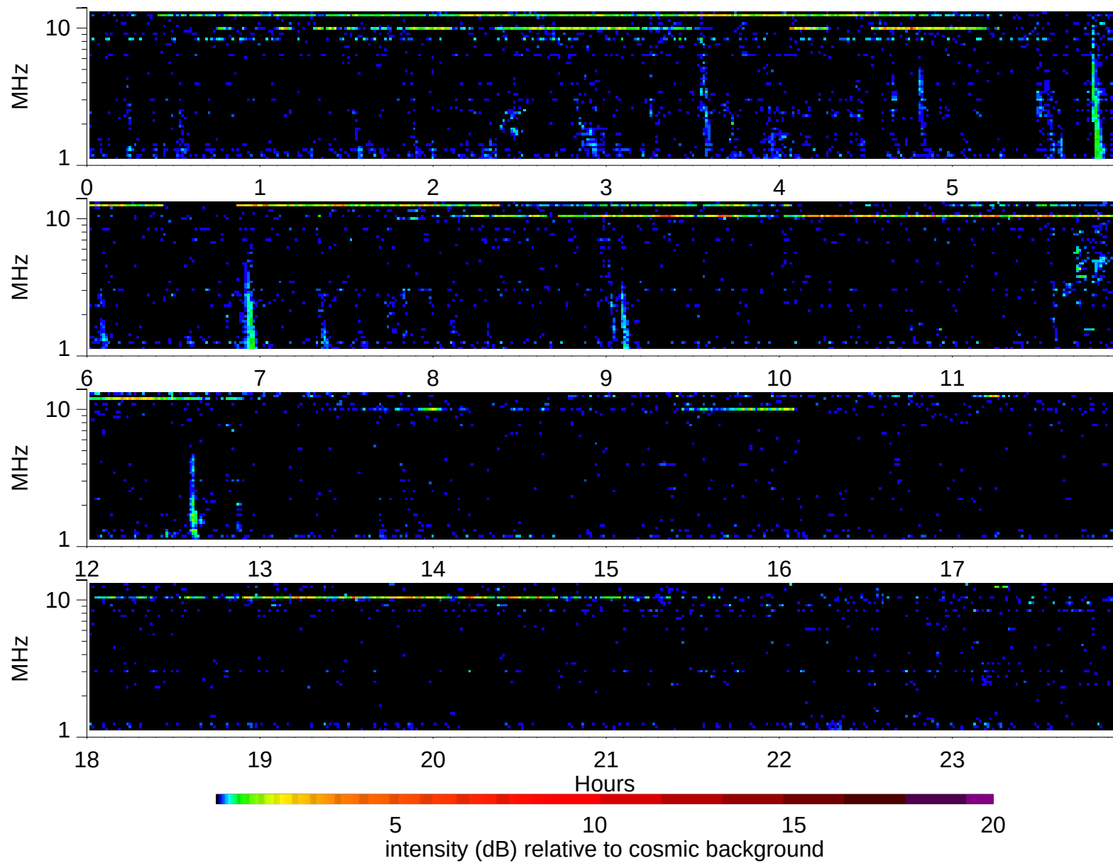
Wind Waves RAD2 receiver: 2006/4/7
