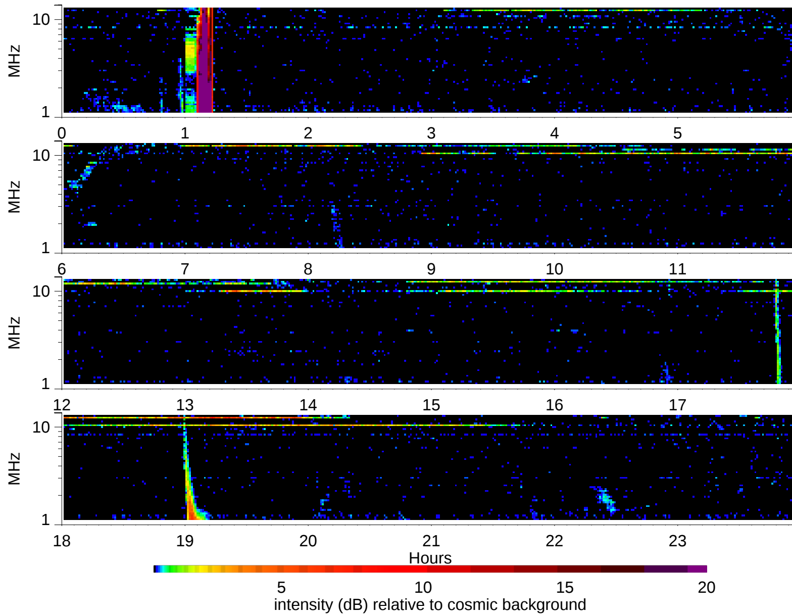
Wind Waves RAD2 receiver: 2006/4/10
