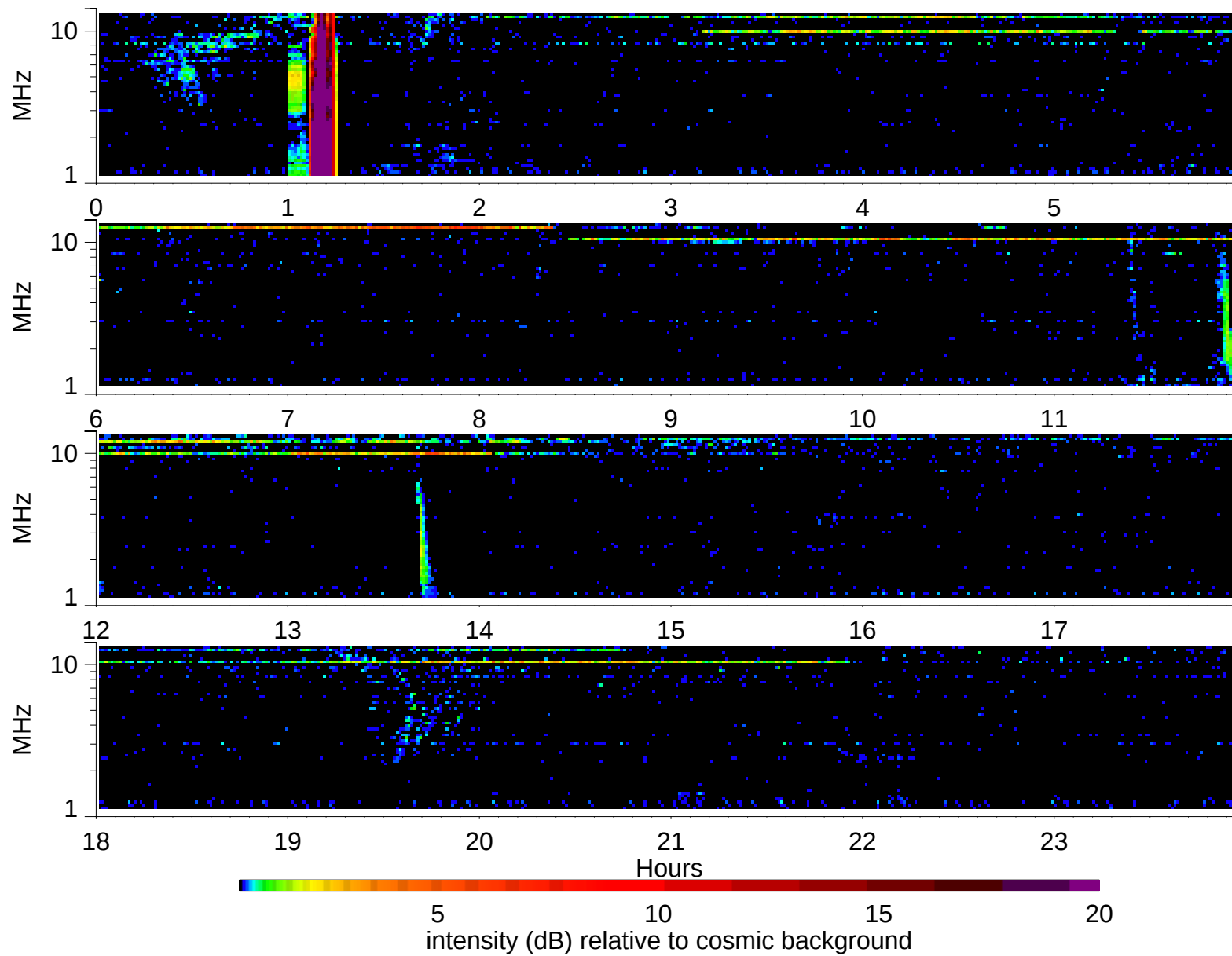
Wind Waves RAD2 receiver: 2006/4/12
