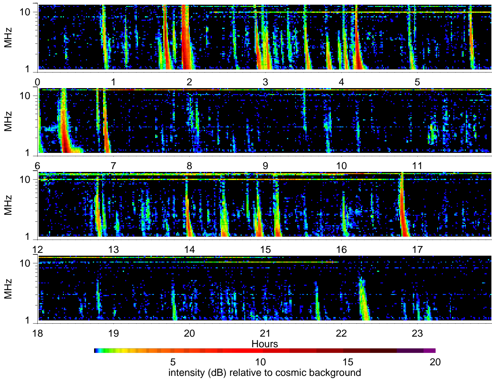
Wind Waves RAD2 receiver: 2006/5/1
