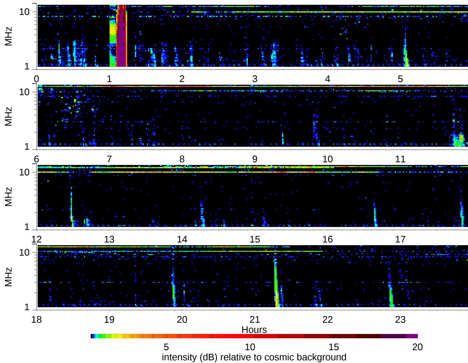
Wind Waves RAD2 receiver: 2006/5/2
