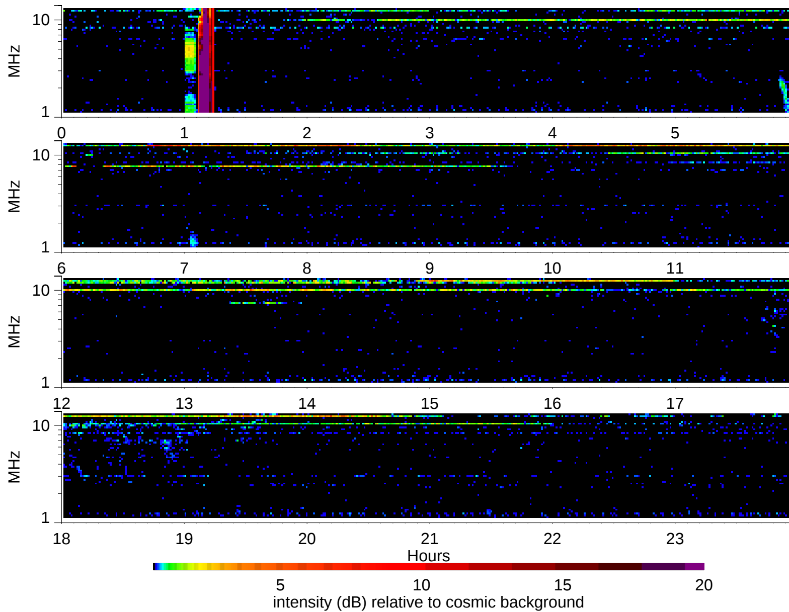
Wind Waves RAD2 receiver: 2006/5/6
